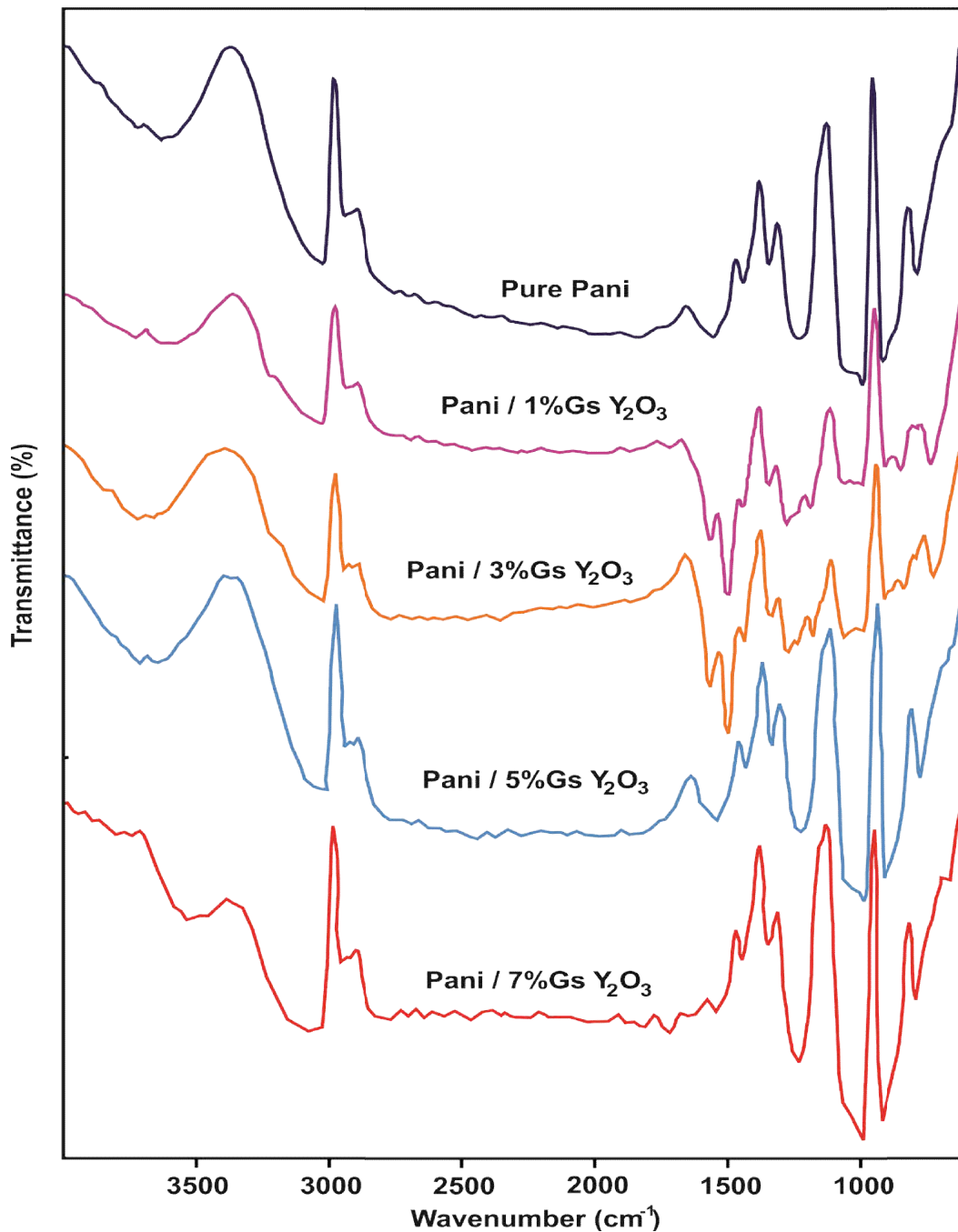
Figure 2: Shows the FTIR spectra of Pure Pani and Pani/ Gs Y_2O_3 nanocomposites
