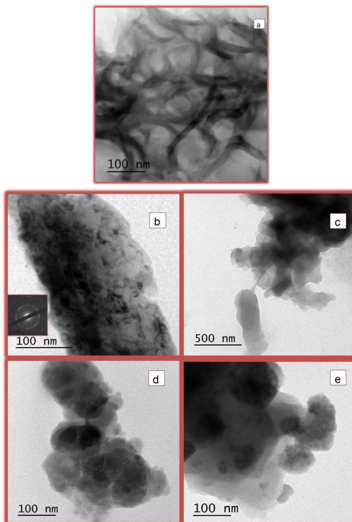
Figure 5: Shows the TEM of (a) Pure Pani (b) Pani/1% Gs Y_2O_3 , (c) Pani/3% Gs Y_2O_3 (d) Pani/5% Gs Y_2O_3 and (e) Pani/7% Gs Y_2O_3 nanocomposites inset of b is for selected area electron diffraction pattern
