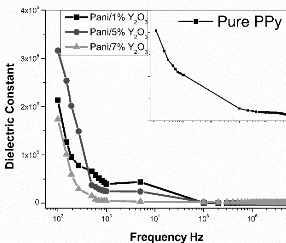
Figure 7: Frequency dependant dielectric constant of Pani/Gs Y_2O_3 composites inset shows for pure Pani
