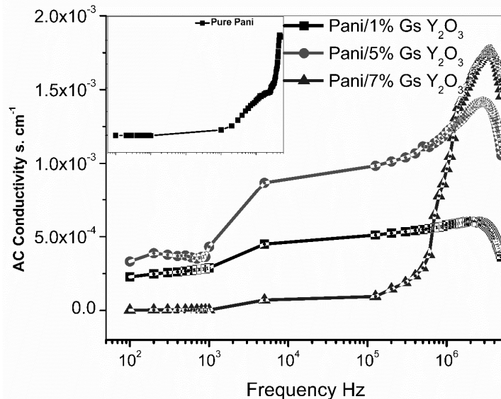
Figure 6: Frequency dependent Ac conductivity of the Pani/ Gs Y 2 O 3 , composites inset shows for pure Pani
