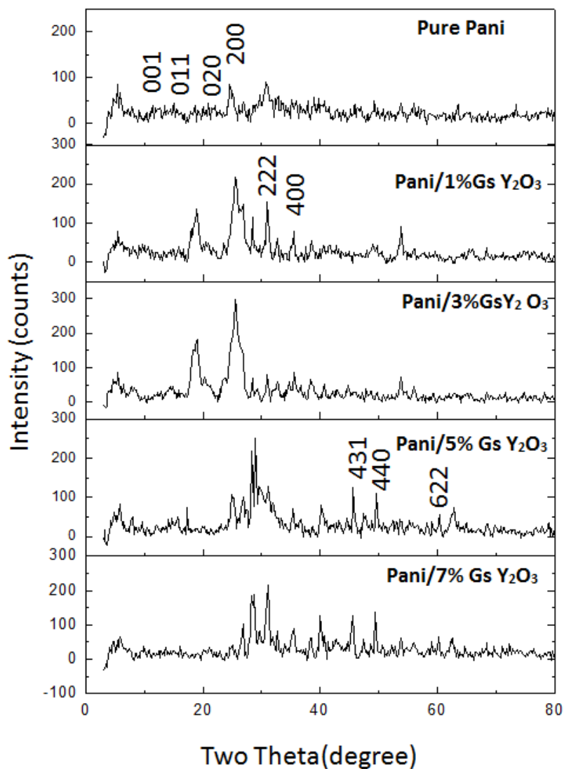
Figure 3: Shows the XRD of pure Pani and Pani/ Gs Y_2O_3 nanocomposites
