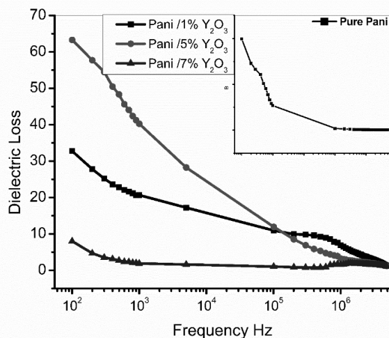
Figure 8: Frequency dependant Dielectric Loss for the Pani/Gs Y_2O_3 composites and inset shows for pure Pani
