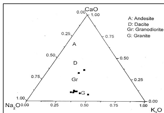
Figure 9: \text{CaO} - \text{Na}_2\text{O} - \text{K}_2\text{O} plots of Bhuban Sandstone (after Le Maitre, 1976)
