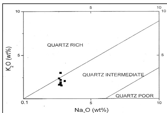
Figure 8: \text{K}_2\text{O} vs. \text{Na}_2\text{O} plot for analyses of Bhuban Sandstone (after Crook, 1974)
