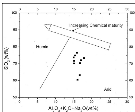
Figure 6: Scatter plot of \text{Al}_2\text{O}_3 + \text{K}_2\text{O} + \text{Na}_2\text{O} vs. \text{SiO}_2 of Bhuban Sandstones (Suttner and Dutta, 1986)
