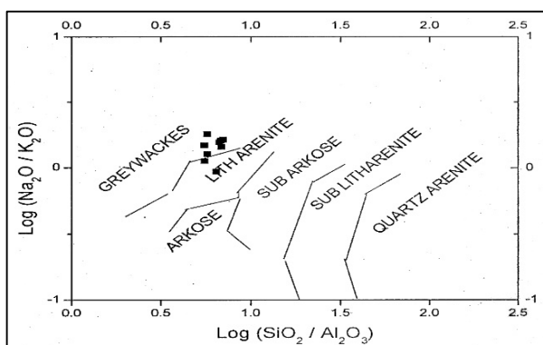
Figure 14: Geochemical classification for Bhuban Sandstones (after Pettijohn et al., 1972)
