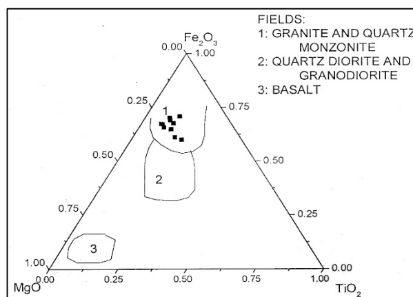
Figure 7: \text{Fe}_2\text{O}_3 - \text{TiO}_2 - \text{MgO} compositional diagram of Bhuban Sandstones (after Condie, 1967)
