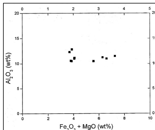
Figure 5: Scatter plot of \text{Fe}_2\text{O}_3 + \text{MgO} vs. \text{Al}_2\text{O}_3 of Bhuban Sandstones (Harker Variation)
