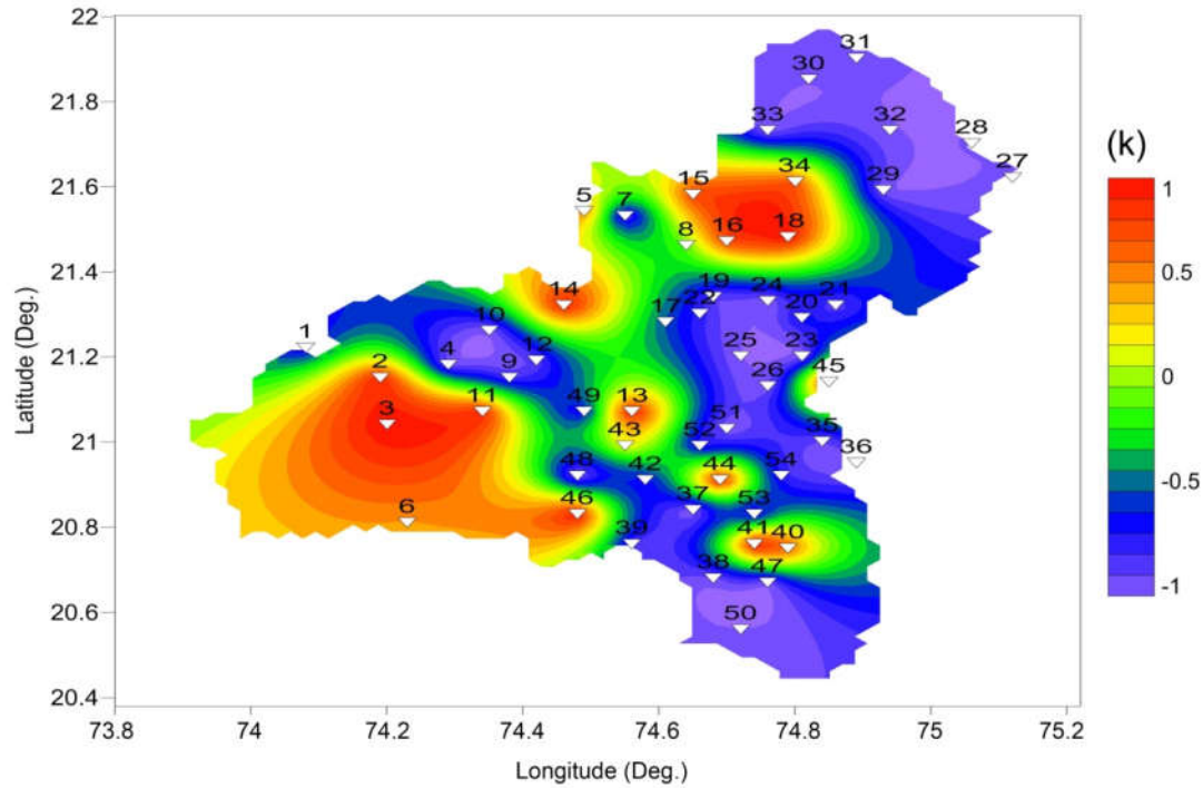
Figure 9: Spatial distribution of reflection coefficient (k) in the study area.
