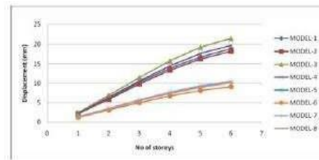
Fig 3: Storey Displacement for G+5 Building
