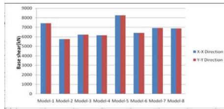
Fig 2 : Comparison of Base Shear for G+5 and G+15 Building
