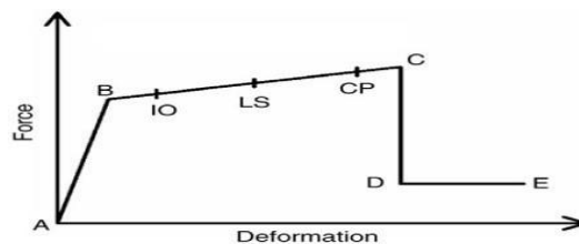
Fig b: load deformation curve
