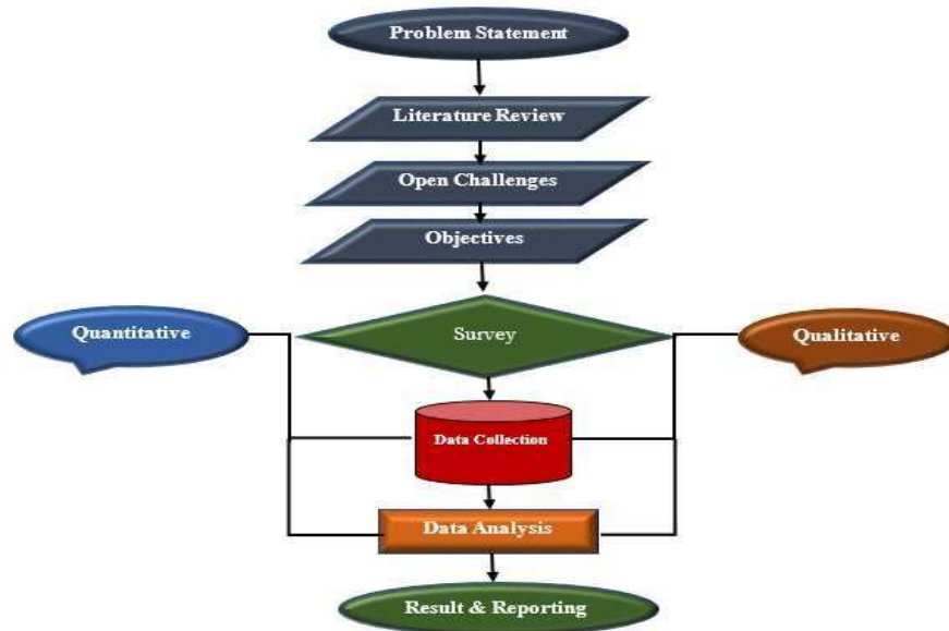
Figure 1. Research Methodology
