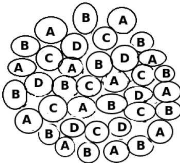
Fig. 3: Compact hexagonal configuration of isometric circles.
