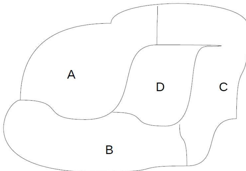
Fig. 1: Regions in a planar domain.
