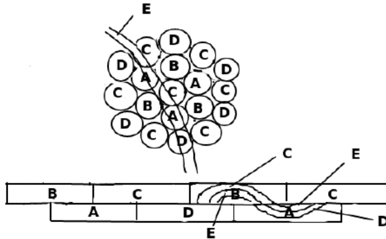
Fig. 4: Interweaving of a ribboned region with a hexagonal set of isometric circles and a brick model.
