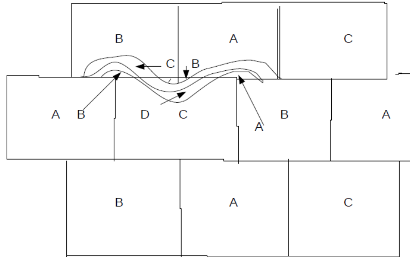
Fig. 2: Interweaving of two ribboned regions with a brick model.
