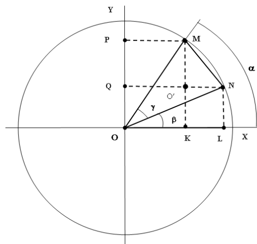
Figure 4: The initial position of the material triangle \triangle MON in the coordinate system XOY . The mobile radii \overline{OM} , \overline{ON} and segment \overline{MN} are the sides of the triangle \triangle MON . Length of the segment \overline{MN} is constant. The relationship between the variable quantities \alpha and \beta has the following form: \gamma = \alpha - \beta where \gamma = \text{const} . Values of quantities are neutral numbers not equal to zero.
