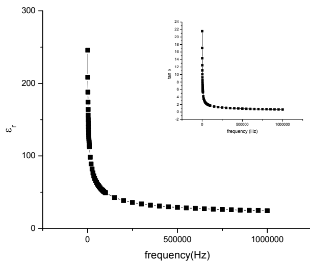
Figure 4: Frequency variation of \epsilon_r and \tan \delta of BTTV at room temp \text{Ba}_5\text{TbTi}_3\text{V}_2\text{O}_{30}
