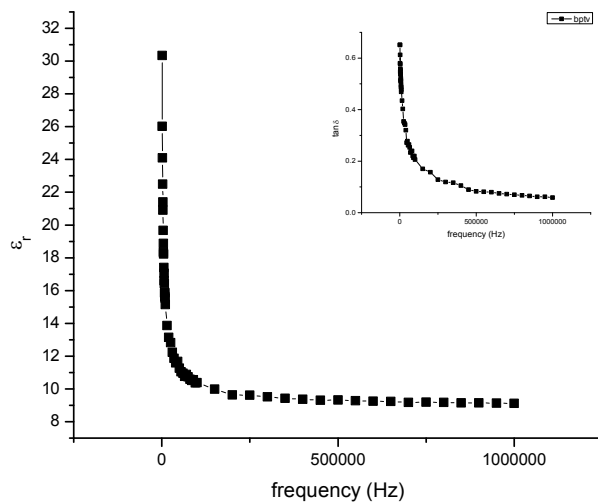
Figure 3: Frequency variation of \epsilon_r and \tan \delta of BPTV at room temp \text{Ba}_5\text{PrTi}_3\text{V}_2\text{O}_{30}
