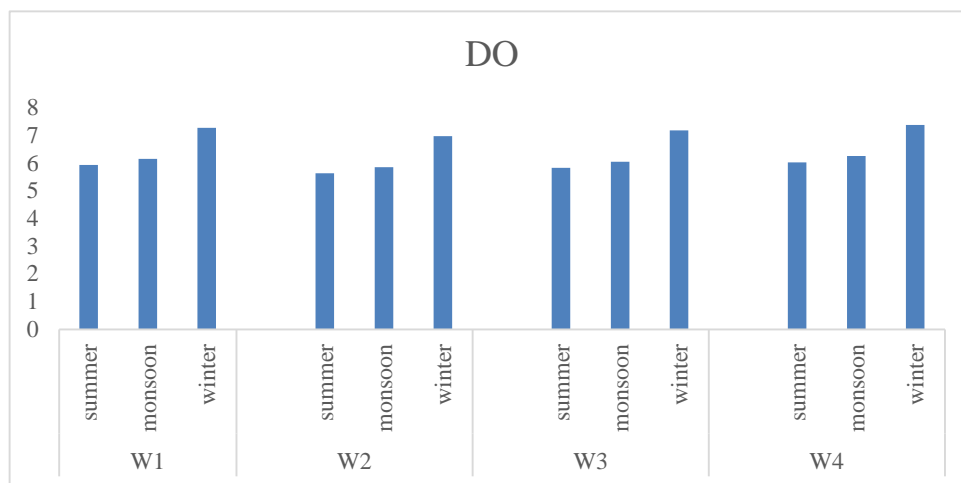
Figure no. 4: Seasonal investigation of DO at station W1, W2, W3 and W4 in Wainganga river.
