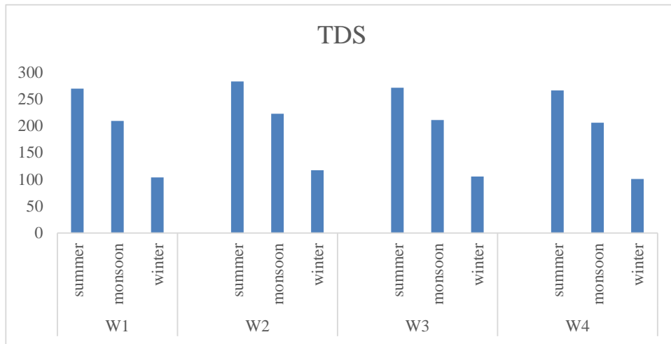
Figure no. 2: Seasonal investigation of EC at station W1, W2, W3 and W4 in Wainganga river.
