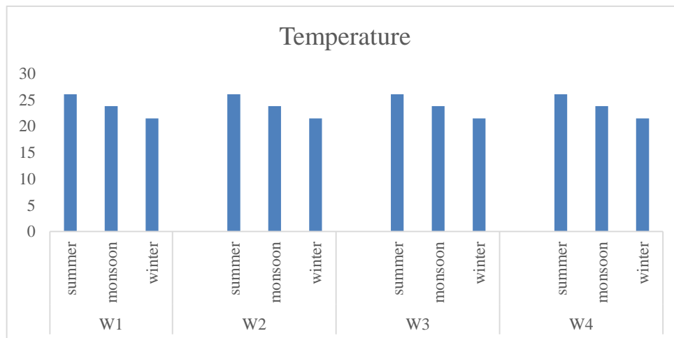
Figure no. 3: Seasonal investigation of Temperature at station W1, W2, W3 and W4 in Wainganga river.
